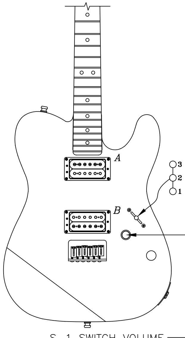
S-1 SWITCH VOLUME POT (UP & DOWN)
