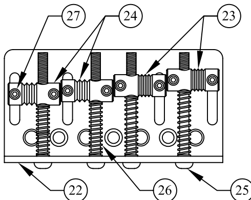
BRIDGE ASSEMBLY
